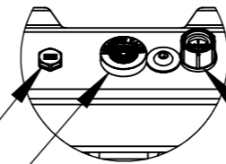
PRV Option Gore Membrane Vent PRV Option AGM Breather Valve PRV Option Humidity Indicator
